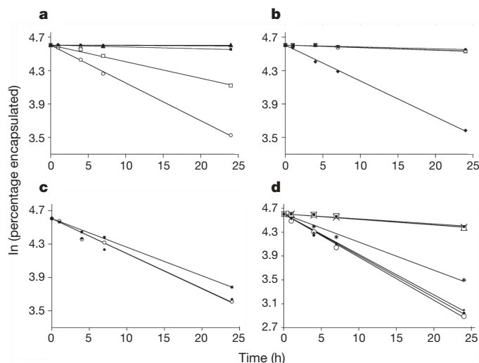
Figure 3 | Time courses of nucleotide permeation through fatty acid based membranes. a , Nucleotide permeation across MA:GMM membranes. Filled square, AMP; open square, AMP + 3 mM MgCl 2 ; filled circle, ADP; open circle, ADP + 3 mM MgCl 2 ; filled triangle, ATP; open triangle, ATP + 3 mM MgCl 2 . b , Permeation of AMP derivatives across MA:GMM membranes. Filled circle, adenosine-5'-monophosphate; open circle, 2'-deoxyadenosine-5'-monophosphate; open square, 2'-amino-2',3'-dideoxyadenosine-5'-monophosphate; filled diamond, 2'-deoxyadenosine-5'-phosphorimidazolidine. c , Permeability of activated nucleotides across MA:GMM membranes. Filled square, adenosine-5'-phosphorimidazolidine; filled circle, 2'-amino-2',3'-dideoxyadenosine-5'-phosphorimidazolidine; open circle, 3'-amino-3'-deoxyadenosine-5'-phosphorimidazolidine. d , Nucleotide permeation across DA:DOH:GMD and DA:DOH membranes. Filled square, AMP; open square, dAMP; X, 2'-amino-2',3'-dideoxyadenosine-5'-monophosphate and asterisk, adenosine-5'-phosphorimidazolidine; filled circle, 2'-deoxyadenosine-5'-phosphorimidazolidine; open circle, 2'-amino-2',3'-dideoxyadenosine-5'-phosphorimidazolidine. All are for 4:1:1 DA:DOH:GMD membranes except for the asterisk, which is 2:1 DA:DOH.
