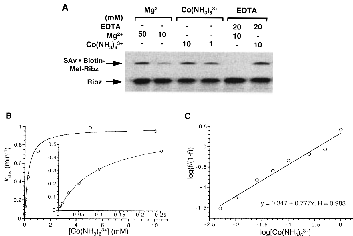
FIGURE 7: (A) Comparison of ribozyme activity in the presence of Mg 2+ or Co(NH 3 ) 6 3+ . Reactions were incubated for 1 min at pH 8.0. (B) Catalytic activity of ribozyme (X = OH) vs Co(NH 3 ) 6 3+ concentration in the presence of 1 mM spermidine. Inset shows activity below 0.25 mM of Co(NH 3 ) 6 3+ . Fitting the data to the equation k_{\text{obs}} = k_{\text{obs}}^{\text{max}}[\text{Co}(\text{NH}_3)_6^{3+}]/(K_d + [\text{Co}(\text{NH}_3)_6^{3+}]) yielded a K_d and k_{\text{obs}}^{\text{max}} shown in Table 1. (C) Hill analysis of the data in panel B.
