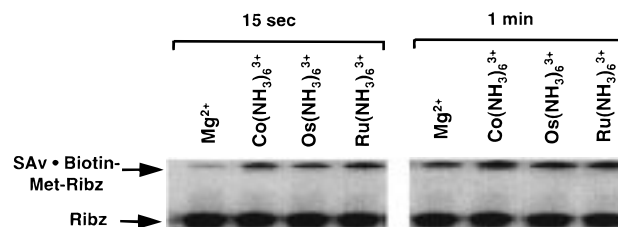
FIGURE 9: Comparison of ribozyme activity in the presence of 10 mM Mg 2+ or metal(III) hexammine.
