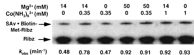
FIGURE 8: Comparison of ribozyme activity in the presence of Mg 2+ or Co(NH 3 ) 6 3+ or both ( t = 15 \text{ s} ). k_{\text{obs}} were determined as described in Materials and Methods.
