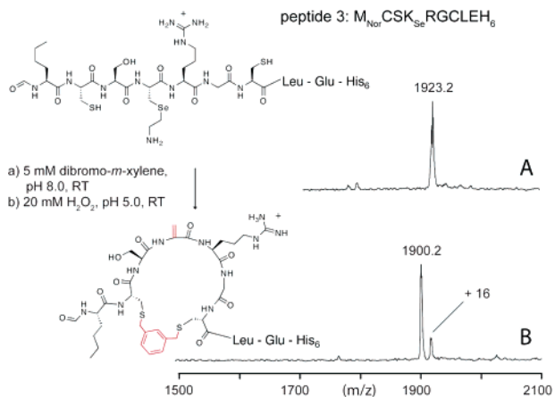
Figure 2. Incorporation of \Delta Ala into a cyclic scaffold. Two concomitant S_N2 reactions between two peptide-borne thiols (A, m_{\text{calc}} = 1923.7 Da) and one equivalent of \alpha, \alpha' -dibromo- m -xylene lead to peptide cyclization. Possible side products, such as the linear adduct of two equivalents of xylene and one peptide, are not observed (B, m_{\text{calc}} = 1900.8 Da). A minor signal 16 Da higher than the expected mass indicates partial sulfoxidation of the newly formed thioethers by the conditions used for \Delta Ala formation.
