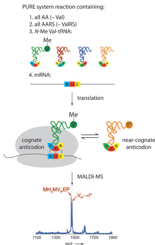
Figure 1. Assay to screen for codons that direct efficient and faithful incorporation of an N -Me AA into a short peptide (MH 6 MX m EP, X m = N -Me AA), using N -Me Val and the GUC codon as an example. In-vitro translation reactions using the PURE system were carried out with 1) total tRNA that had been enzymatically precharged with Val and chemically N -methylated ( N -Me Val-tRNA), 2) all 19 other natural amino acid/aminoacyl-tRNA synthetase pairs, and 3) mRNA encoding MH 6 MX m EP where N -Me Val incorporation was directed by the GUC codon. Translation products were analyzed by MALDI-TOF MS to assess the efficiency of N -Me Val incorporation (i.e. absence of truncation products) and the extent of misincorporation of non-cognate amino acids. In the example above, using the GUC codon resulted in significant misincorporation of Ile (I; the asterisk represents an isotope label to break the mass degeneracy with N -Me Val). After repeating the assay for each of the remaining Val codons, the codon(s) that yielded the N -methyl peptide with no misincorporation or truncation products were judged to be optimal.
